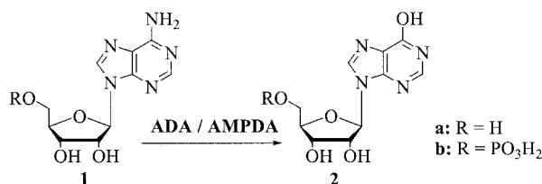
Scheme 1. ADA- and AMPDA-catalyzed deamination of adenosine ( 1a ) and 5'-adenylic acid ( 1b )
