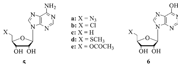
Figure 2. Structure of adenosine 5a-e and inosine derivatives 6a-e
