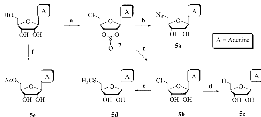
Scheme 2. Reagents and conditions: (a) \text{SOCl}_2 , Py, \text{CH}_3\text{CN} , 0\text{ }^\circ\text{C} ; (b) \text{NaN}_3 , DMF, 80\text{ }^\circ\text{C} ; (c) aq. MeOH, room temp; (d) \text{LiEt}_3\text{BH} , DMSO, room temp; (e) \text{CH}_3\text{SNa} , DMF, room temp; (f) Candida antarctica , vinyl acetate, THF, room temp.
