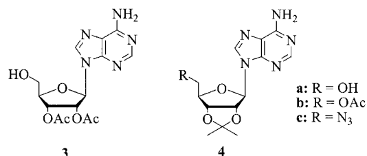
Figure 1. Structure of 2',3'- O -diacetyladenosine ( 3 ) and 2',3'- O -isopropylideneadenosines 4a-c
